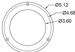
PR35 Mounting Flange
